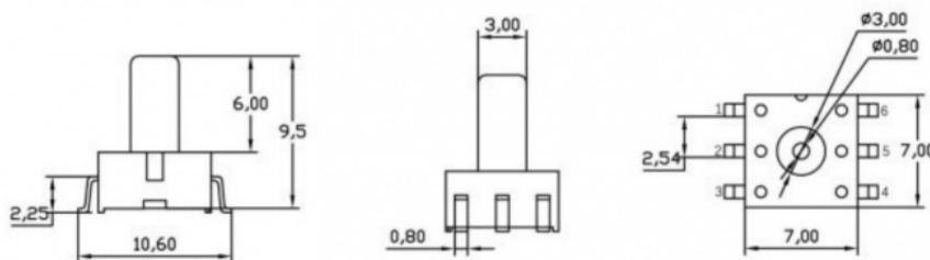
(SOP outline)
