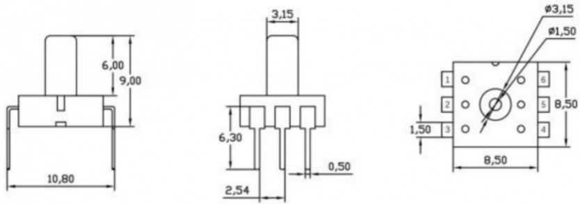
(DIP Outline - R type)
