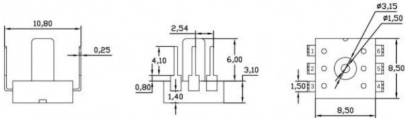
(DIP Outline - F type)
